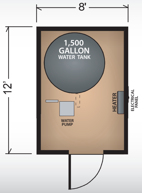
Supply Tank + Enclosure
