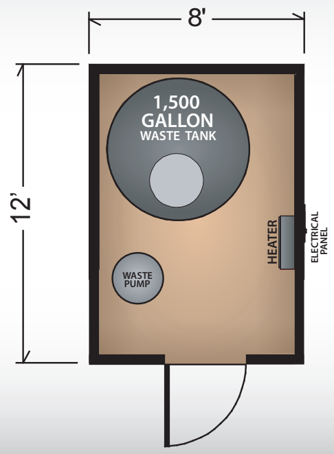
Waste Tank + Enclosure
